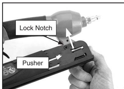
Figure 4. Lifting the pusher into the lock notch.
