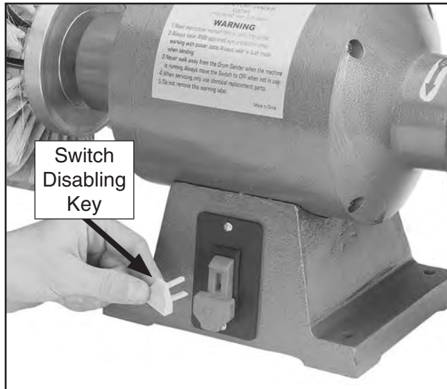
Figure 14. Removing the ON/OFF switch disabling key.
